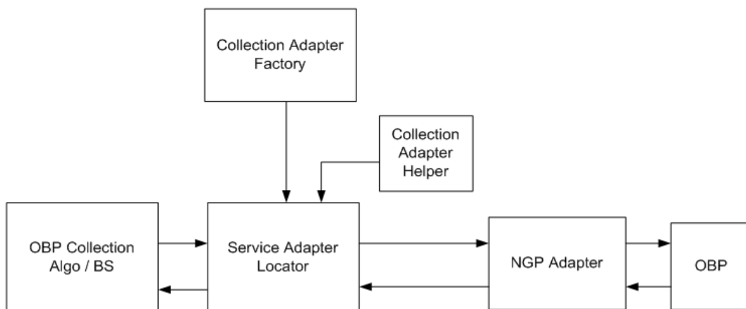
Figure 2–1 Adapter Architecture
